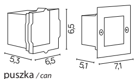
puszka / can
