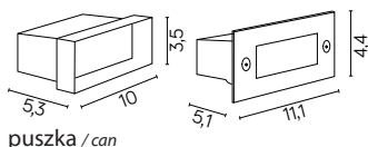
puszka / can
