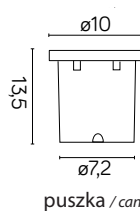
puszka / can
