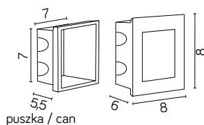
puszka / can
