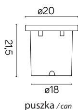
puszka / can
