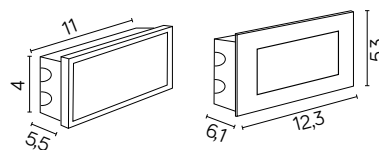
puszka / can
